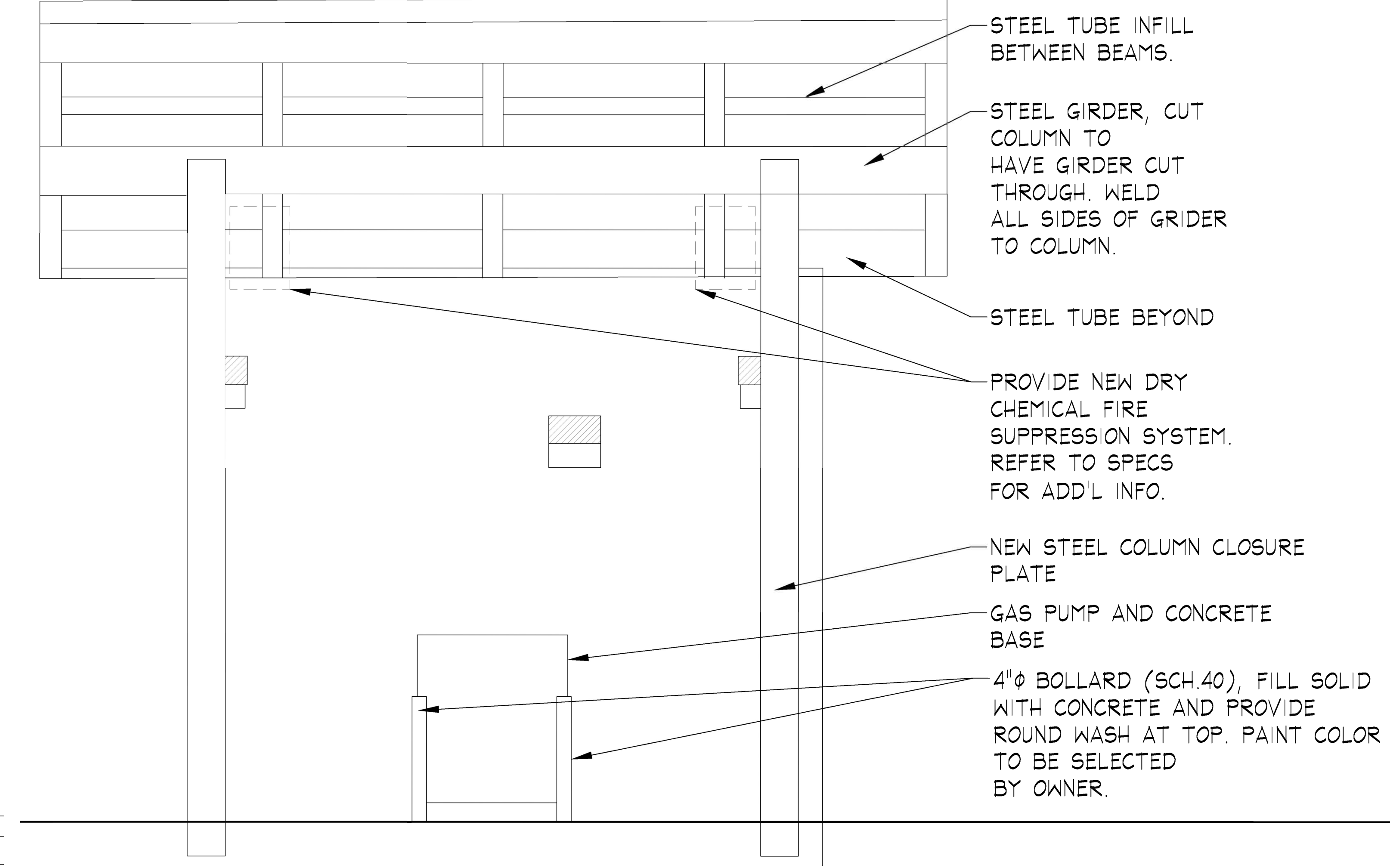
56 CANOPY SOUTH ELEVATION SCALE: 1/2" = 1'-0"
