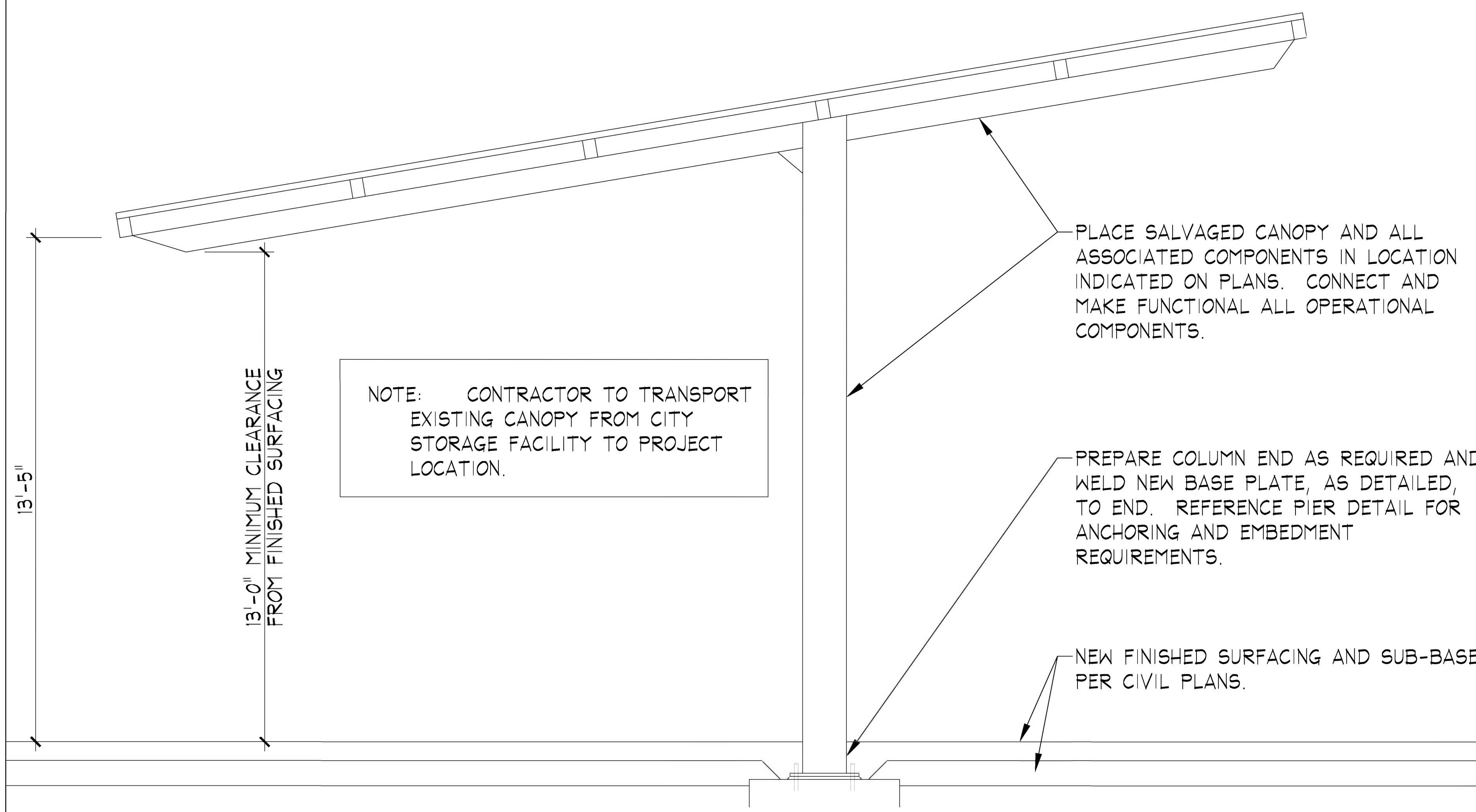
55 CANOPY EAST ELEVATION SCALE: 1/2" = 1'-0"
